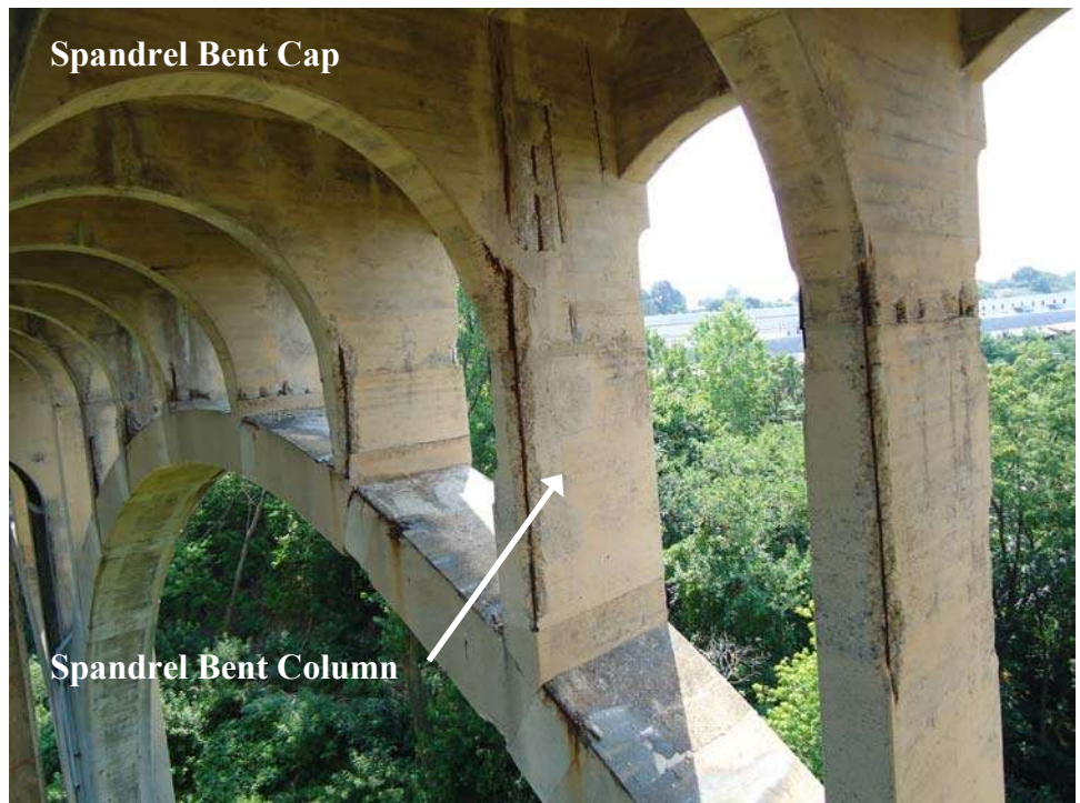
Figure 9.5.13 Spandrel Column Bent Cap Interface
