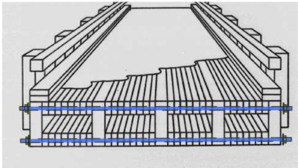
Figure 8.3.7 Typical Section of a Stress-Laminated Timber Box Beam (Source: Barry Dickson, West Virginia University)
