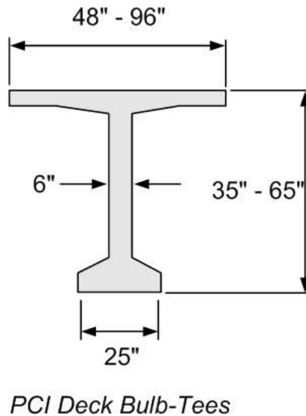
Figure 9.9.6 Cross Section of AASHTO-PCI Bulb-Tee Beams
