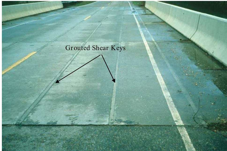
Figure 9.4.6 Top of Deck View of Precast Channel Beam Bridge
