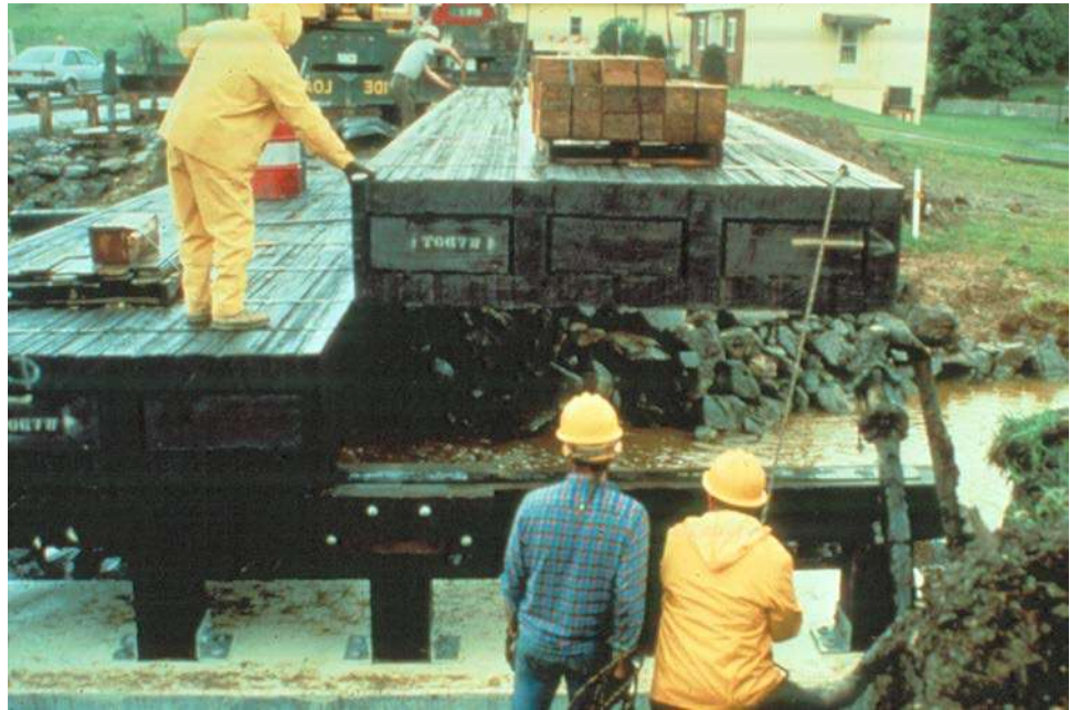
Figure 8.3.8 Stress-Laminated Timber Box Beam Bridge Being Erected
