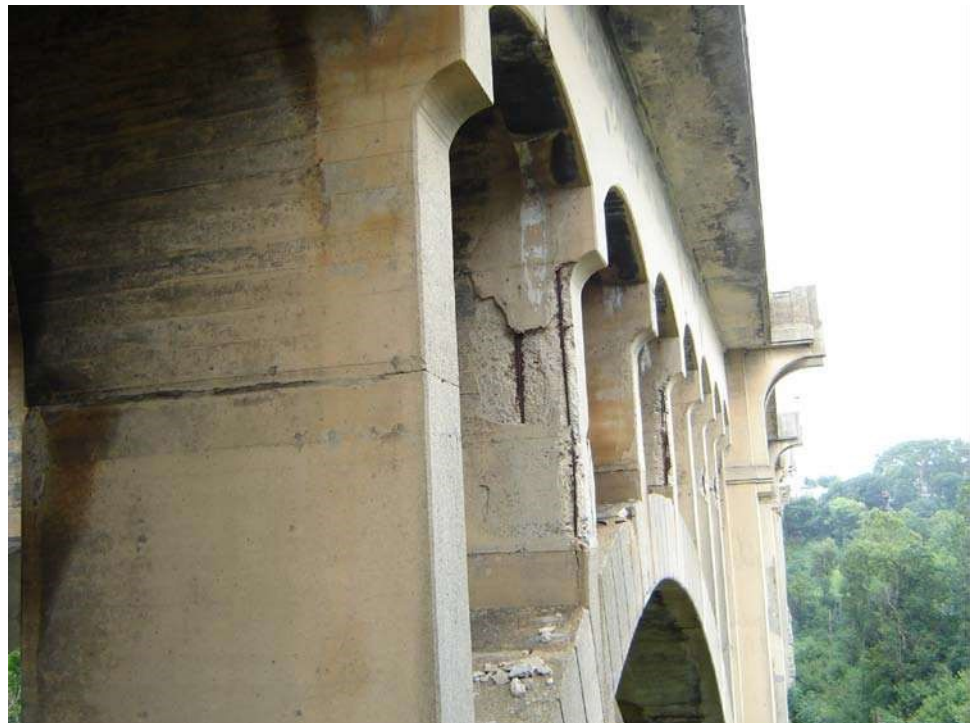
Figure 9.5.16 Severe Scaling and Spalling on a Spandrel Column
